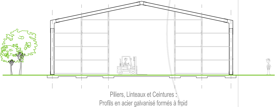
Pignon Principal
