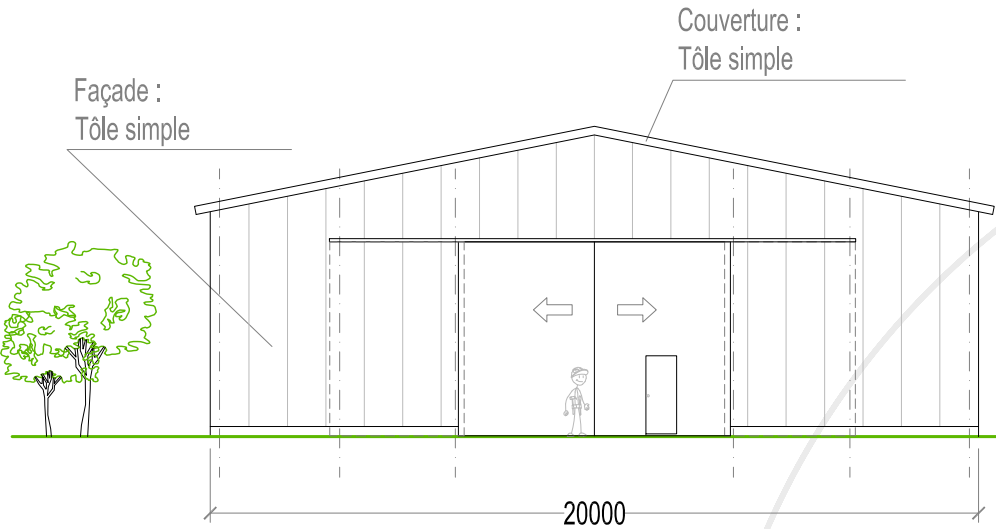
Pignon Principal
